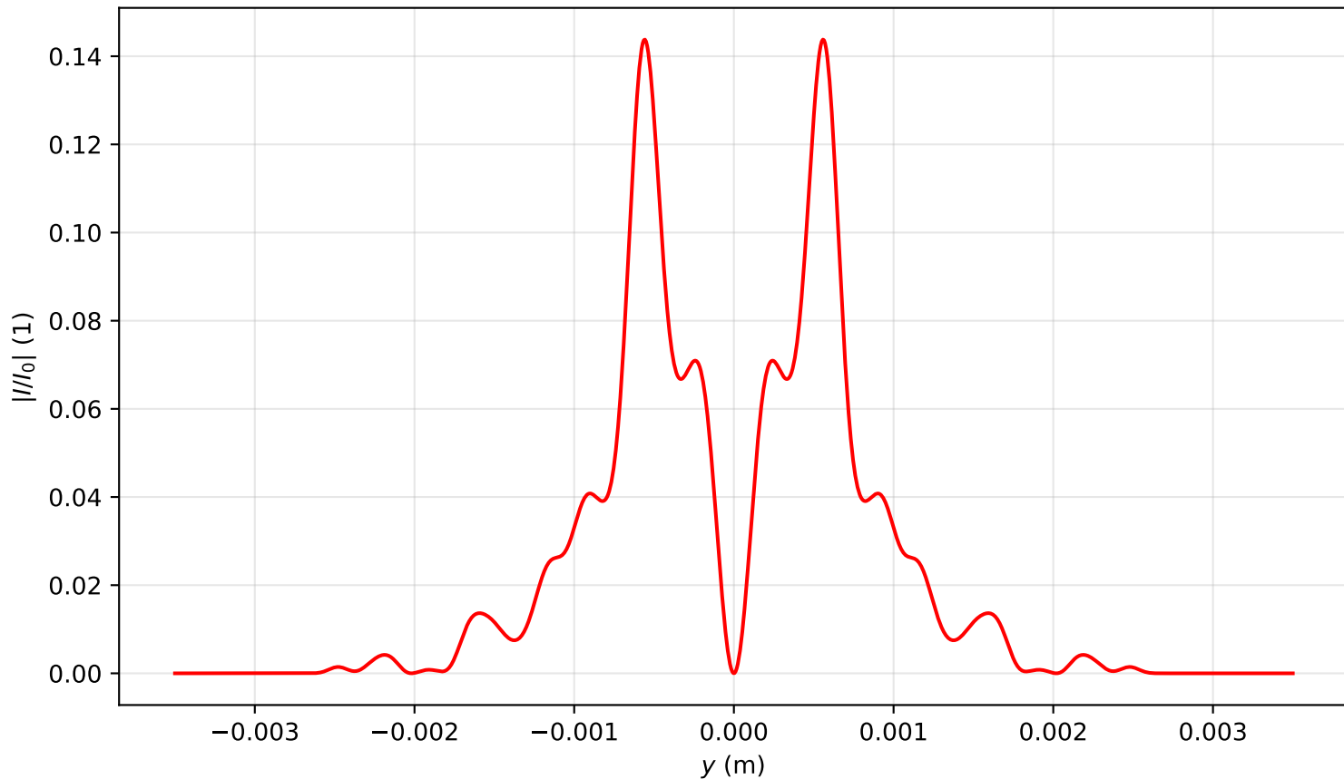
Intensity profile I(x=0, y, z=3.423)/I_0 , P_{in}=7.0P_{cr} , artificial time
